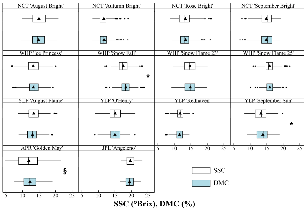
Figure 2. Soluble solids concentration (SSC) and dry matter concentration (DMC) in fourteen stone fruit cultivars (NCT = nectarine; YLP = yellow peach; WHP = white peach; APR = apricot; JPL = Japanese plum) at harvest (n = 200). Boxplots display interquartile range boxes (1st to 3rd quartile) with means (black triangles), medians (vertical lines), highest and lowest observations (whiskers) and outliers (dots). Asterisks (*) represent significant differences between SSC and DMC means based on Student’s t -test ( p < 0.05 ). Section signs (§) represent significant differences between SSC and DMC standard deviations based on Levene’s test ( p < 0.05 ).
